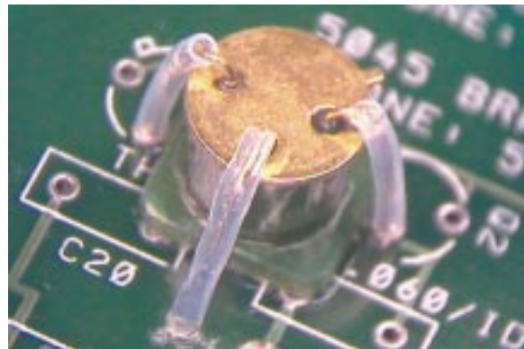
Figure 14 Radial lead component mounted upside down. Note: Insulate leads to avoid contact with component body.
